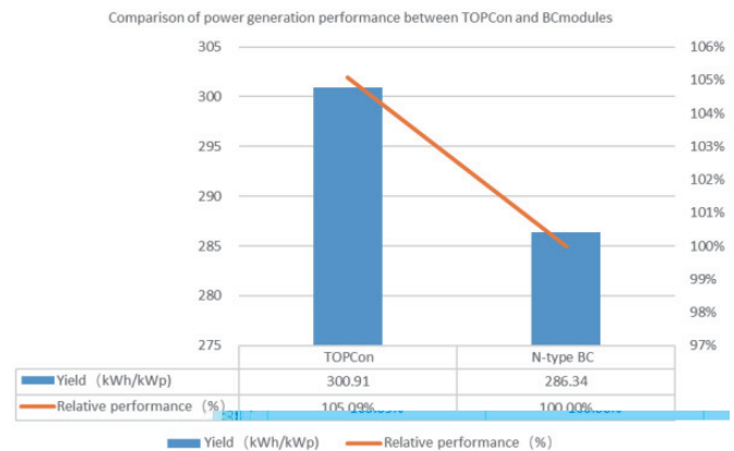
Figure 1: Comparison of power generation per watt between TOPCon and other BC II modules
